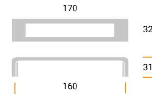
MZ1875 Materiale / Material: Metal Largh. / Width: 32 mm. Lungh. / Length 170 mm. Alt. / Height 31 mm. Interasse / Cd 160 mm.
