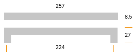
MZA2107 Materiale / Material: Metal Largh. / Width: 8,5 mm. Lungh. / Length 257 mm. Alt. / Height 27 mm. Interasse / Cd 224 mm.
