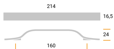
MZA2095 Materiale / Material: Metal Largh. / Width: 16,5 mm. Lungh. / Length 214 mm. Alt. / Height 24 mm. Interasse / Cd 160 mm.
