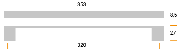
MZA2108 Materiale / Material: Metal Largh. / Width: 8,5 mm. Lungh. / Length 353 mm. Alt. / Height 27 mm. Interasse / Cd 320 mm.
