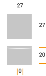
MZ1160 Materiale / Material: Metal Largh. / Width: 27 mm. Lungh. / Length 27 mm. Alt. / Height 20 mm. Interasse / Cd 0 mm.
