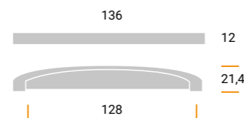
MZ968 Materiale / Material: Metal Largh. / Width: 12 mm. Lungh. / Length 136 mm. Alt. / Height 21,4 mm. Interasse / Cd 128 mm.
