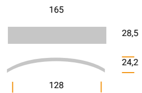
MZ1198 Materiale / Material: Metal Largh. / Width: 28,5 mm. Lungh. / Length 165 mm. Alt. / Height 24,2 mm. Interasse / Cd 128 mm.
