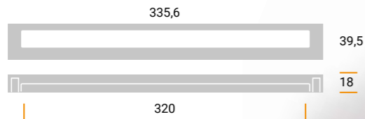
MZ1470 Materiale / Material: Metal Largh. / Width: 39,5 mm. Lungh. / Length 335,5 mm. Alt. / Height 18 mm. Interasse / Cd 320 mm.
