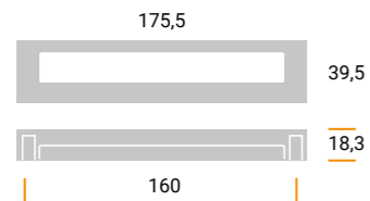
MZ1463 Materiale / Material: Metal Largh. / Width: 39,5 mm. Lungh. / Length 175,5 mm. Alt. / Height 18,3 mm. Interasse / Cd 160 mm.
