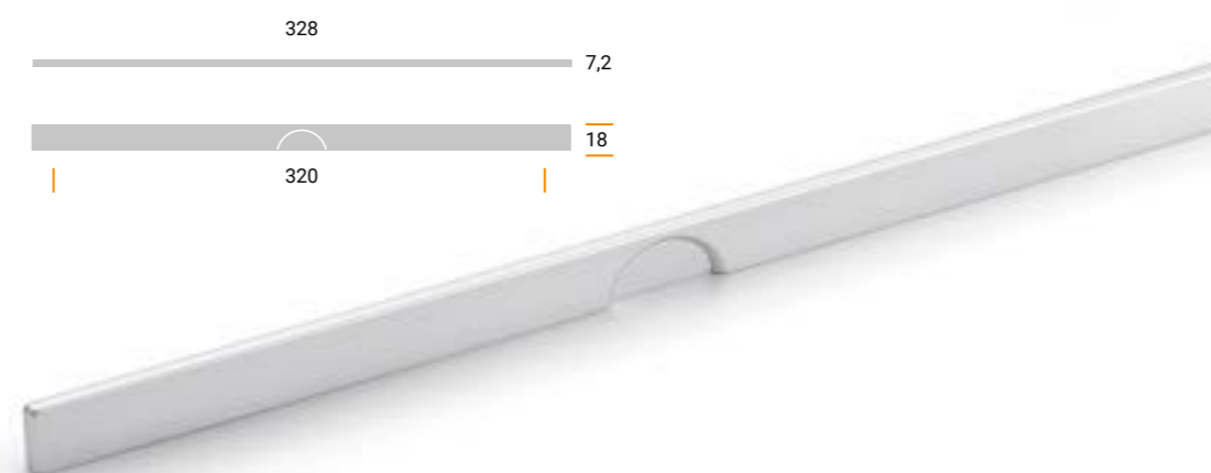
MZ1230 Materiale / Material: Metal Largh. / Width: 7,2 mm. Lungh. / Length 328 mm. Alt. / Height 18 mm. Interasse / Cd 320 mm.
