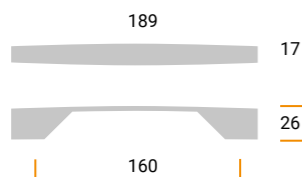
MZ1655 Materiale / Material: Metal Largh. / Width: 17 mm. Lungh. / Length 189 mm. Alt. / Height 26 mm. Interasse / Cd 160 mm.
