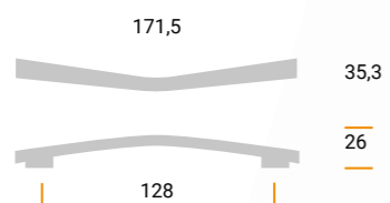
MZ1777 Materiale / Material: Metal Largh. / Width: 35,3 mm. Lungh. / Length 171,5 mm. Alt. / Height 26 mm. Interasse / Cd 128 mm.
