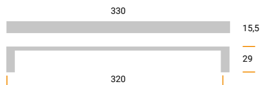
MZ2057 Materiale / Material: Metal Largh. / Width: 15,5 mm. Lungh. / Length 330 mm. Alt. / Height 29 mm. Interasse / Cd 320 mm.
