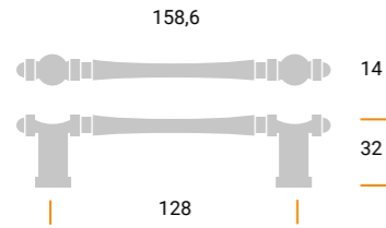
MZ2319 Materiale / Material: Metal Largh. / Width: 14 mm. Lungh. / Length 158,6 mm. Alt. / Height 32 mm. Interasse / Cd 128 mm.
