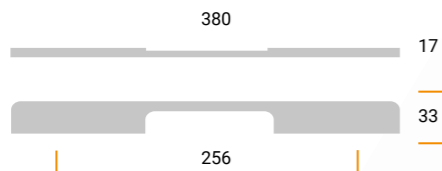
MZA1954 Materiale / Material: Metal Largh. / Width: 17 mm. Lungh. / Length 380 mm. Alt. / Height 33 mm. Interasse / Cd 256 mm.
