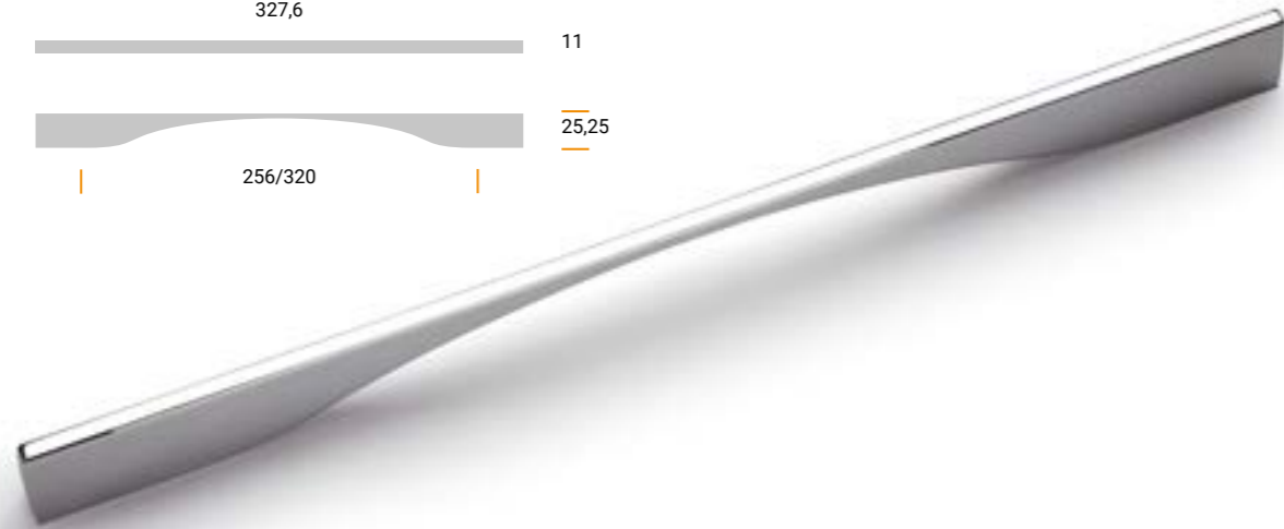
MZ1661 Materiale / Material: Metal Largh. / Width: 11 mm. Lungh. / Length 327,6 mm. Alt. / Height 25,25 mm. Interasse / Cd 256/320 mm.
