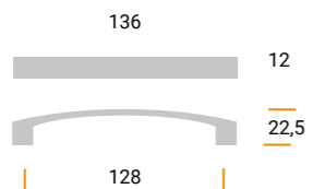
MZ1107 Materiale / Material: Metal Largh. / Width: 12 mm. Lungh. / Length 136 mm. Alt. / Height 22,5 mm. Interasse / Cd 128 mm.
