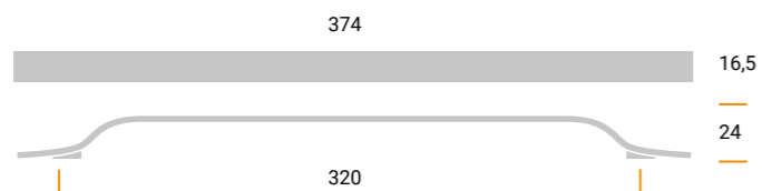
MZA2098 Materiale / Material: Metal Largh. / Width: 16,5 mm. Lungh. / Length 374 mm. Alt. / Height 24 mm. Interasse / Cd 320 mm.
