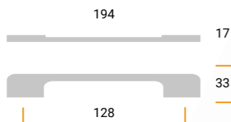
MZA1950 Materiale / Material: Metal Largh. / Width: 17 mm. Lungh. / Length 194 mm. Alt. / Height 33 mm. Interasse / Cd 128 mm.
