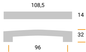
MZ1762 Materiale / Material: Metal Largh. / Width: 14 mm. Lungh. / Length 108,5 mm. Alt. / Height 32 mm. Interasse / Cd 96 mm.
