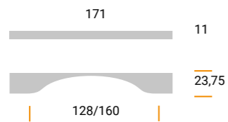
MZ1659 Materiale / Material: Metal Largh. / Width: 11 mm. Lungh. / Length 171 mm. Alt. / Height 23,75 mm. Interasse / Cd 128/160 mm.
