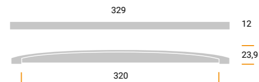
MZ971 Materiale / Material: Metal Largh. / Width: 12 mm. Lungh. / Length 329 mm. Alt. / Height 23,9 mm. Interasse / Cd 320 mm.
