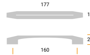
MZ1935 Materiale / Material: Metal Largh. / Width: 17 mm. Lungh. / Length 177 mm. Alt. / Height 28 mm. Interasse / Cd 160 mm.
