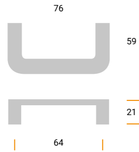
MZ2299 Materiale / Material: Metal Largh. / Width: 59 mm. Lungh. / Length 76 mm. Alt. / Height 21 mm. Interasse / Cd 64 mm.
