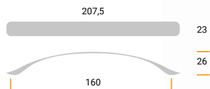
MZA2140 Materiale / Material: Metal Largh. / Width: 23 mm. Lungh. / Length 207,5 mm. Alt. / Height 26 mm. Interasse / Cd 160 mm.
