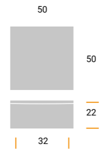
MZ1148 Materiale / Material: Metal Largh. / Width: 50 mm. Lungh. / Length 50 mm. Alt. / Height 22 mm. Interasse / Cd 32 mm.
