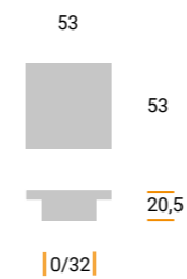
MZ1535 Materiale / Material: Metal Largh. / Width: 53 mm. Lungh. / Length 53 mm. Alt. / Height 20,5 mm. Interasse / Cd 0/32 mm. Doppio interasse / Double centre distance
