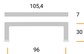
MZ988 Materiale / Material: Metal Largh. / Width: 7 mm. Lungh. / Length 105,4 mm. Alt. / Height 30 mm. Interasse / Cd 96 mm.
