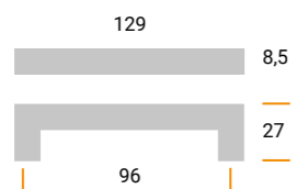
MZA2104 Materiale / Material: Metal Largh. / Width: 8,5 mm. Lungh. / Length 129 mm. Alt. / Height 27 mm. Interasse / Cd 96 mm.
