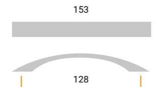
MZA1910 Materiale / Material: Metal Largh. / Width: 25 mm. Lungh. / Length 153 mm. Alt. / Height 27 mm. Interasse / Cd 128 mm.
