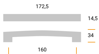
MZ1764 Materiale / Material: Metal Largh. / Width: 14,5 mm. Lungh. / Length 172,5 mm. Alt. / Height 34 mm. Interasse / Cd 160 mm.
