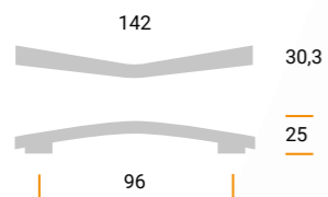
MZ1776 Materiale / Material: Metal Largh. / Width: 30,3 mm. Lungh. / Length 142 mm. Alt. / Height 25 mm. Interasse / Cd 96 mm.
