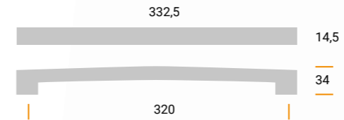
MZ1766 Materiale / Material: Metal Largh. / Width: 14,5 mm. Lungh. / Length 332,5 mm. Alt. / Height 34 mm. Interasse / Cd 320 mm.
