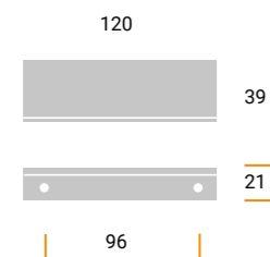
MZ1558/F Materiale / Material: Metal Largh. / Width: 39 mm. Lungh. / Length 120 mm. Alt. / Height 21 mm. Interasse / Cd 96 mm. (2 fori / 2 holes)
