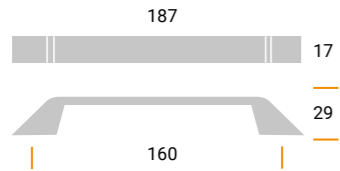
MZ1945 Materiale / Material: Metal Largh. / Width: 17 mm. Lungh. / Length 187 mm. Alt. / Height 29 mm. Interasse / Cd 160 mm.
