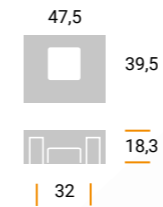
MZ1460 Materiale / Material: Metal Largh. / Width: 47,5 mm. Lungh. / Length 39,5 mm. Alt. / Height 18,3 mm. Interasse / Cd 32 mm.
