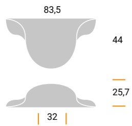
MZ1940 Materiale / Material: Metal Largh. / Width: 44 mm. Lungh. / Length 83,5 mm. Alt. / Height 25,7 mm. Interasse / Cd 32 mm.
