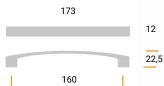
MZ1108 Materiale / Material: Metal Largh. / Width: 12 mm. Lungh. / Length 173 mm. Alt. / Height 22,5 mm. Interasse / Cd 160 mm.
