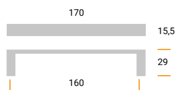
MZ2055 Materiale / Material: Metal Largh. / Width: 15,5 mm. Lungh. / Length 170 mm. Alt. / Height 29 mm. Interasse / Cd 160 mm.
