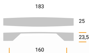
MZ1643 Materiale / Material: Metal Largh. / Width: 25 mm. Lungh. / Length 183 mm. Alt. / Height 23,5 mm. Interasse / Cd 160 mm.
