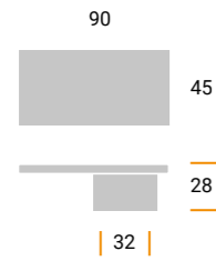
MZ1625 Materiale / Material: Metal Largh. / Width: 45 mm. Lungh. / Length 90 mm. Alt. / Height 28 mm. Interasse / Cd 32 mm.
