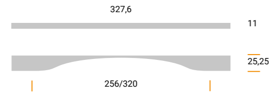
MZ1661 Materiale / Material: Metal Largh. / Width: 11 mm. Lungh. / Length 327,6 mm. Alt. / Height 25,25 mm. Interasse / Cd 256/320 mm.
