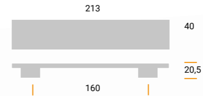
MZ1538 Materiale / Material: Metal Largh. / Width: 40 mm. Lungh. / Length 213 mm. Alt. / Height 20,5 mm. Interasse / Cd 160 mm.
