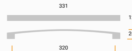
MZ1110 Materiale / Material: Metal Largh. / Width: 12 mm. Lungh. / Length 331 mm. Alt. / Height 26 mm. Interasse / Cd 320 mm.
