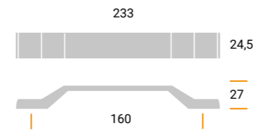
MZ1870 Materiale / Material: Metal Largh. / Width: 24,5 mm. Lungh. / Length 233 mm. Alt. / Height 27 mm. Interasse / Cd 160 mm.
