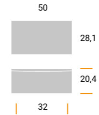
MZ1161 Materiale / Material: Metal Largh. / Width: 28,1 mm. Lungh. / Length 50 mm. Alt. / Height 20,4 mm. Interasse / Cd 32 mm.
