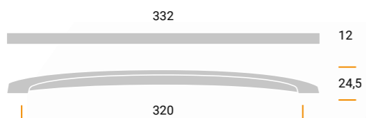
MZ971c Materiale / Material: Metal Largh. / Width: 12 mm. Lungh. / Length 332 mm. Alt. / Height 24,5 mm. Interasse / Cd 320 mm.
