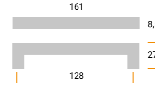
MZA2106 Materiale / Material: Metal Largh. / Width: 8,5 mm. Lungh. / Length 161 mm. Alt. / Height 27 mm. Interasse / Cd 128 mm.
