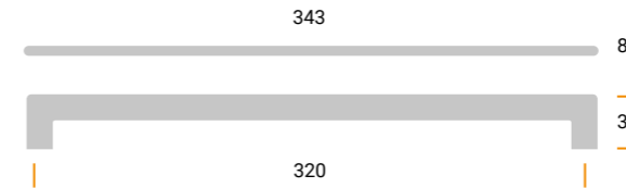
MZ2287 Materiale / Material: Metal Largh. / Width: 8 mm. Lungh. / Length 343 mm. Alt. / Height 34 mm. Interasse / Cd 320 mm.
