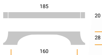
MZ1880 Materiale / Material: Metal Largh. / Width: 20 mm. Lungh. / Length 185 mm. Alt. / Height 28 mm. Interasse / Cd 160 mm.
