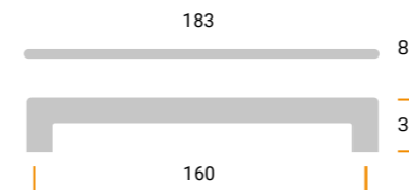
MZ2285 Materiale / Material: Metal Largh. / Width: 8 mm. Lungh. / Length 183 mm. Alt. / Height 34 mm. Interasse / Cd 160 mm.
