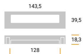
MZ1462 Materiale / Material: Metal Largh. / Width: 39,5 mm. Lungh. / Length 143,5 mm. Alt. / Height 18,3 mm. Interasse / Cd 128 mm.
