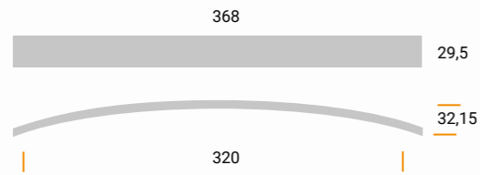
MZ1565 Materiale / Material: Metal Largh. / Width: 29,5 mm. Lungh. / Length 368 mm. Alt. / Height 32,15 mm. Interasse / Cd 320 mm.
