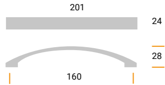
MZA1916 Materiale / Material: Metal Largh. / Width: 24 mm. Lungh. / Length 201 mm. Alt. / Height 28 mm. Interasse / Cd 160 mm.
